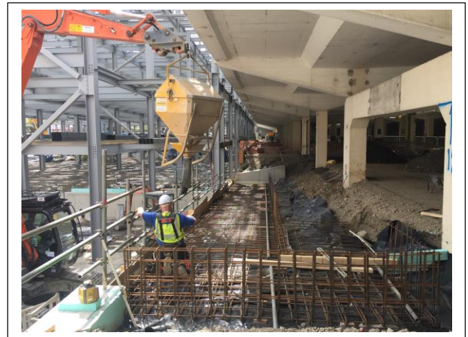
Concrete pour of pedestrian access ramp to undercroft car park.
